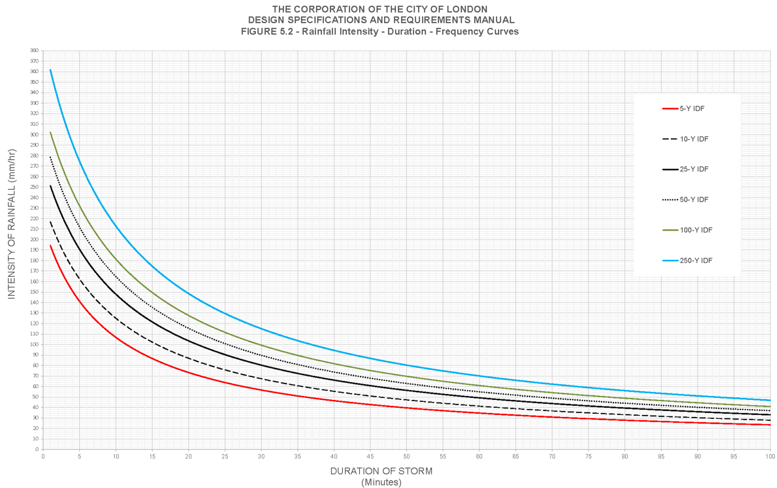
Figure 5.2 Rainfall Intensity-Duration Curves for Storm Sewer Design
