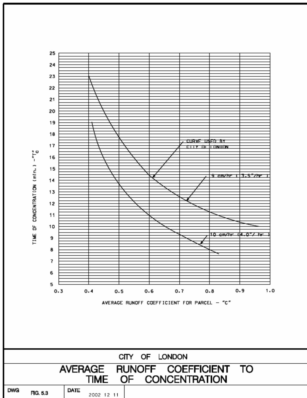
Figure 5.3 Average Runoff Coefficient to Time of Concentration
