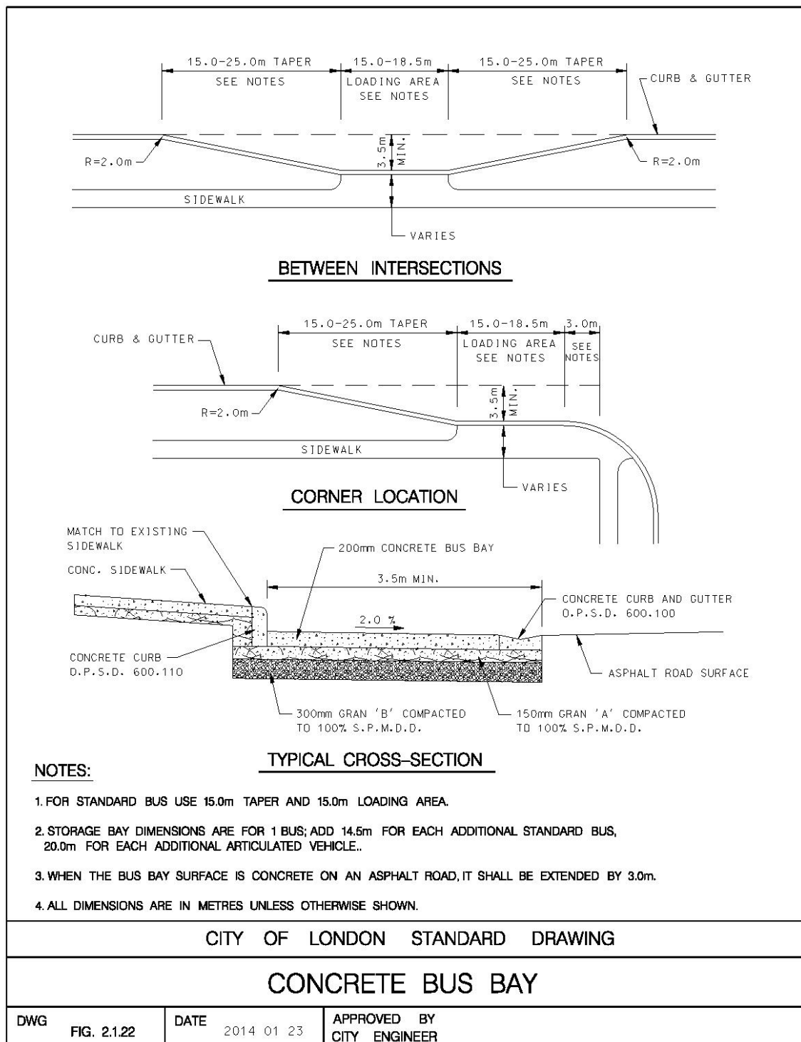
Figure 2.1.22 Concrete Bus Bay
