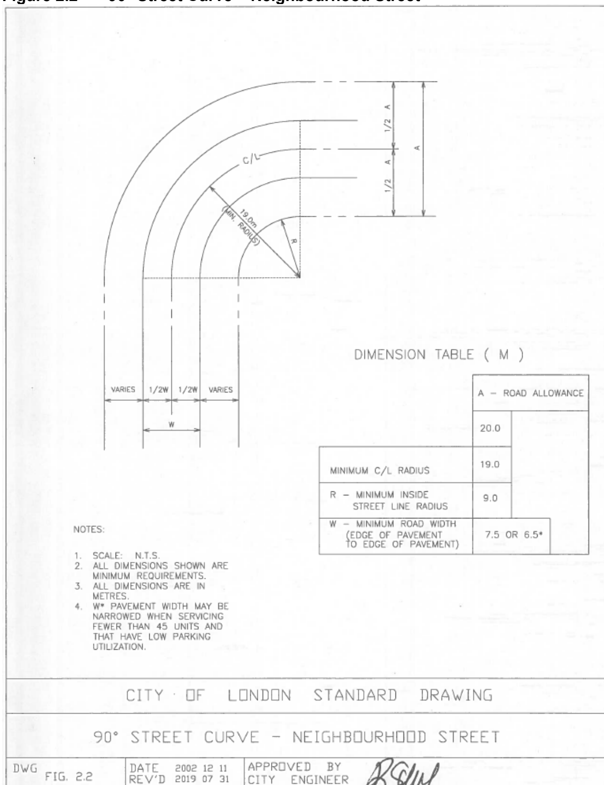
Figure 2.2 90° Street Curve – Neighbourhood Street
