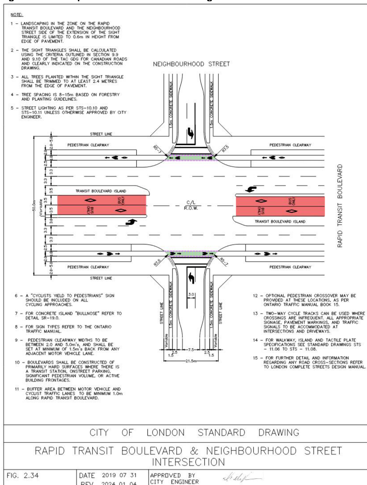
Figure 2.34 Rapid Transit Boulevard & Neighbourhood Street Intersection
