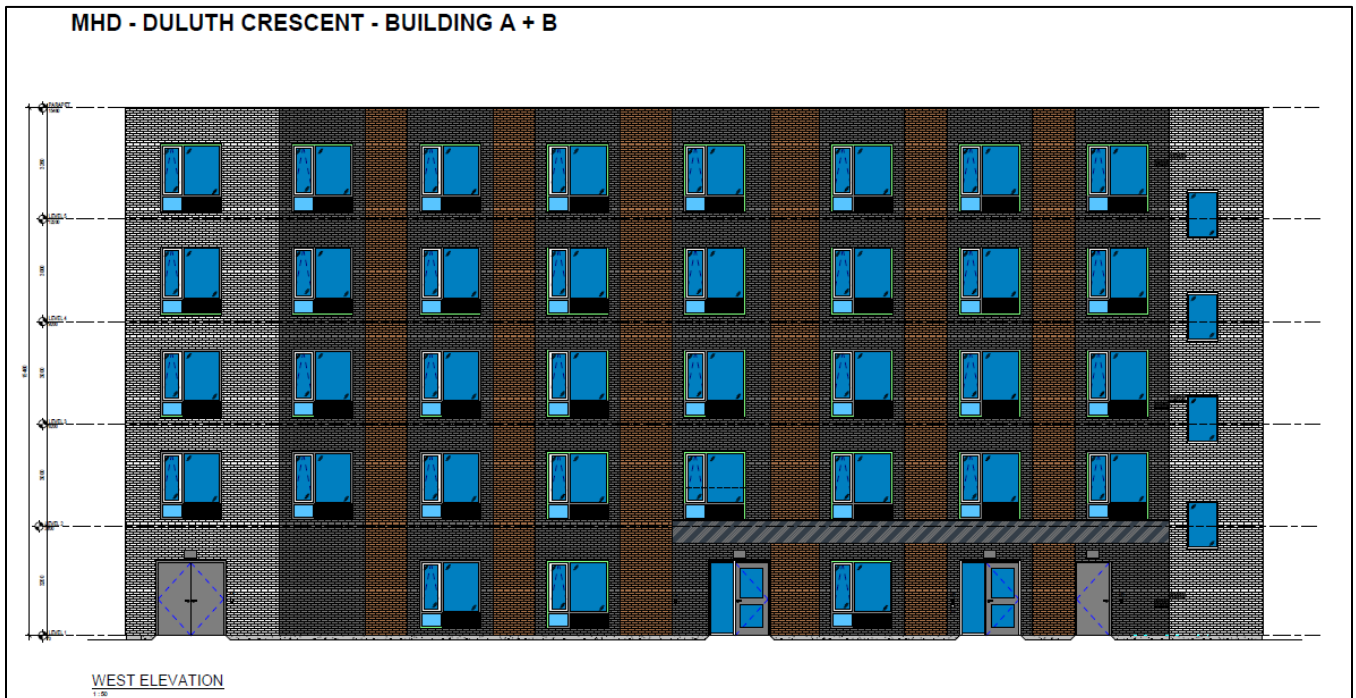
West Elevation proposed development, 1958 Duluth Crescent, Block 5
