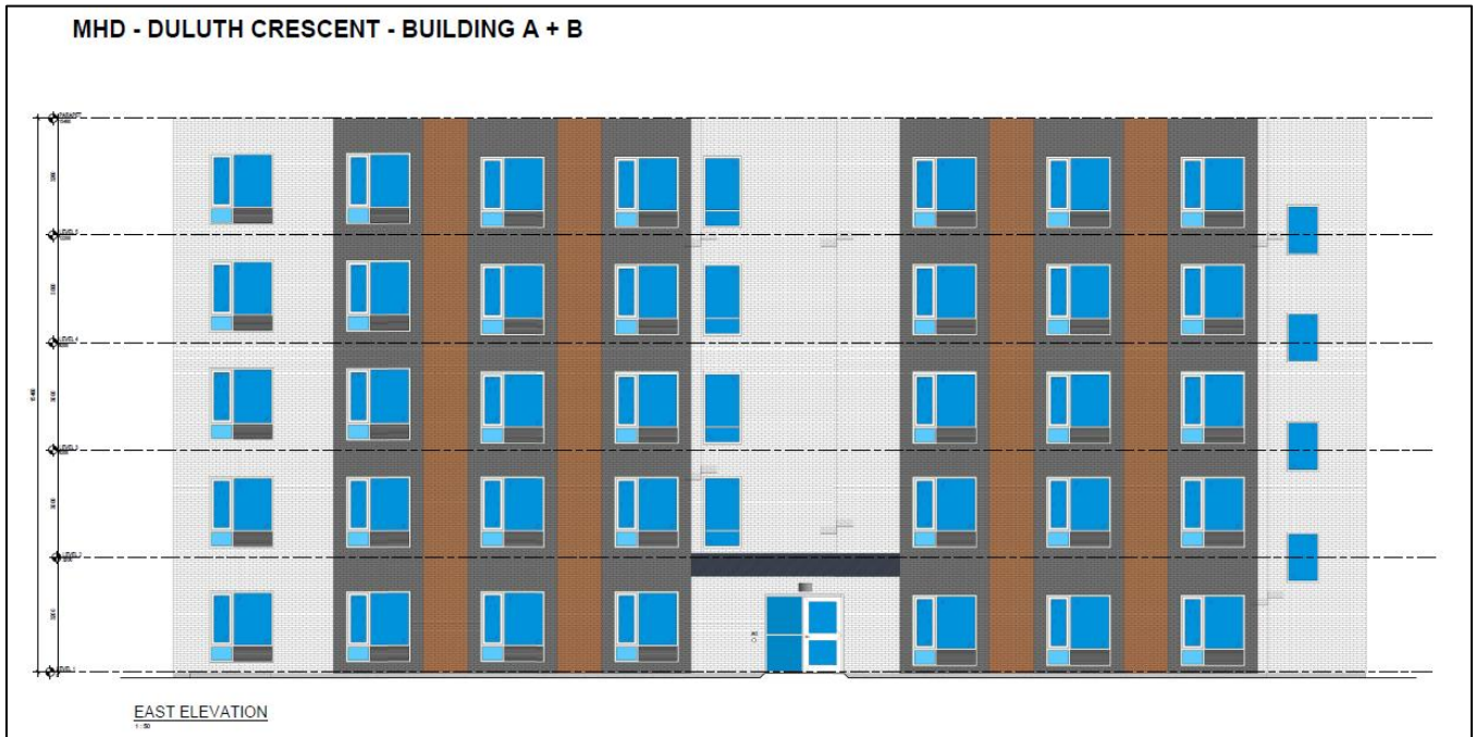
East Elevation proposed development, 1958 Duluth Crescent, Block 5
