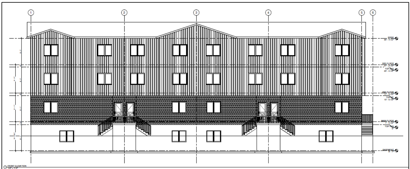
Front Elevation 325 Southdale Road East
