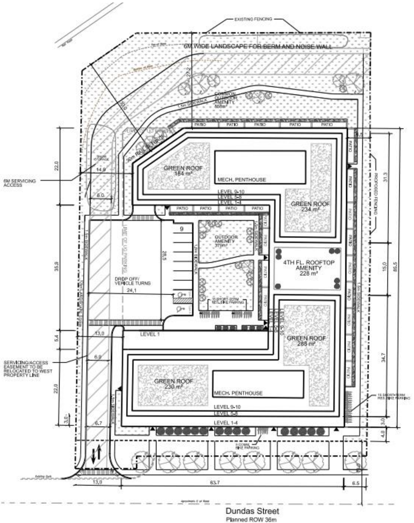
Site Concept Plan 1472 Dundas Street
