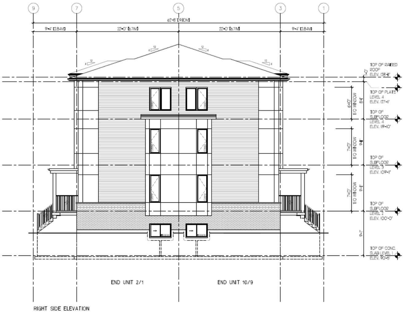
Right Side Elevation 279 Sarnia Road
