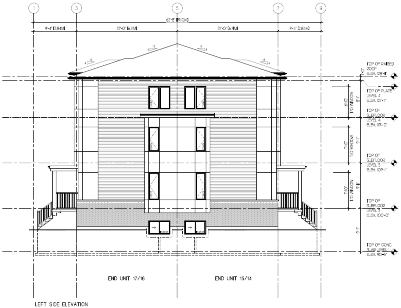
Left Side Elevation 279 Sarnia Road
