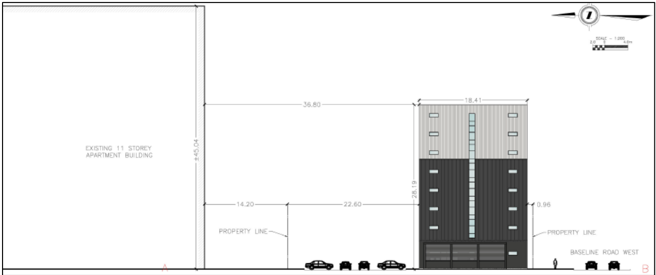
Cross Section 8-storey apartment building, looking east.
