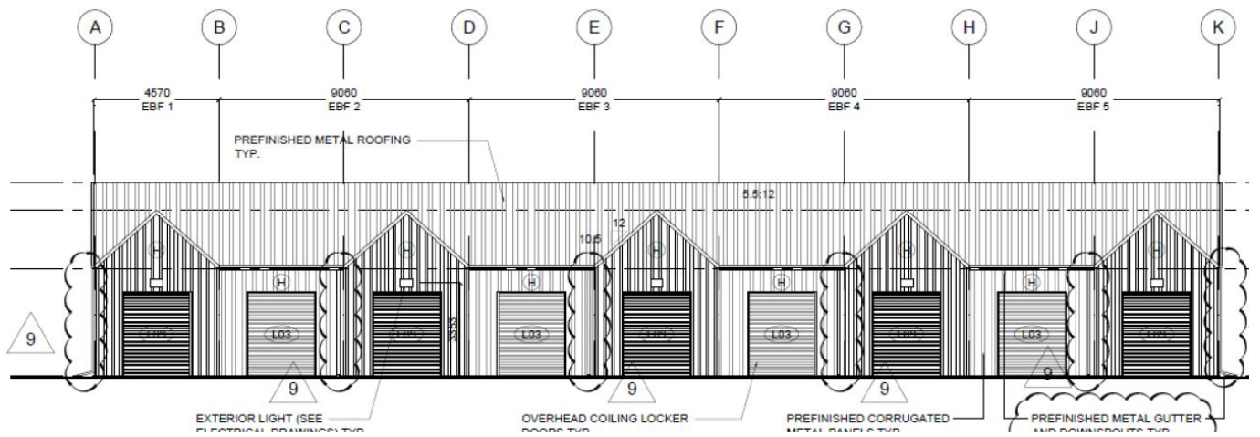
Figure 2: Conceptual Elevation of the proposed outdoor self-storage units
