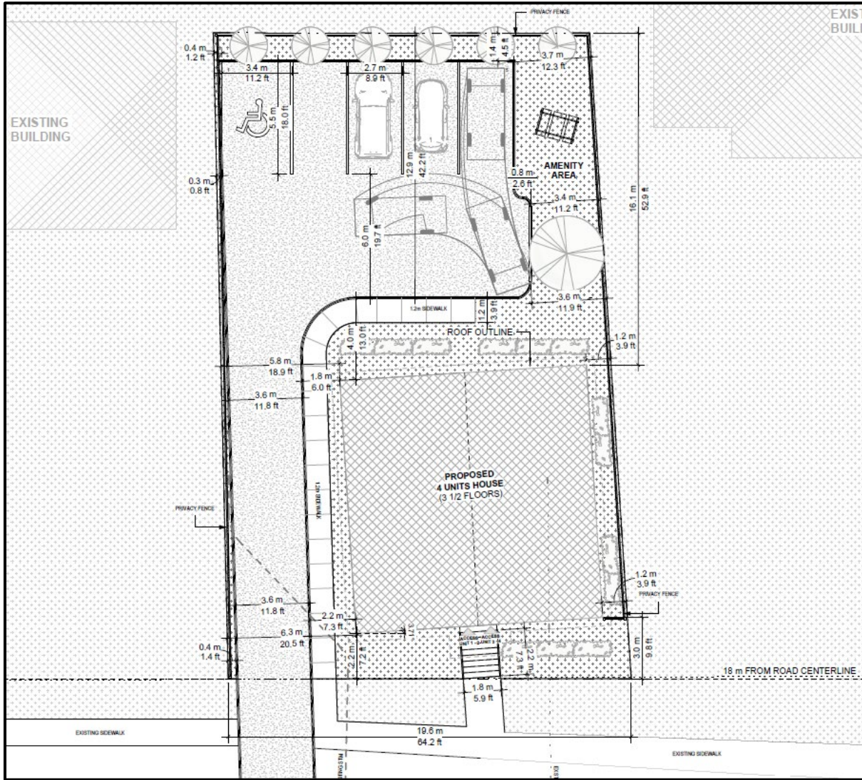
Figure 1. Site Concept Plan for 130 Southdale Road West.
