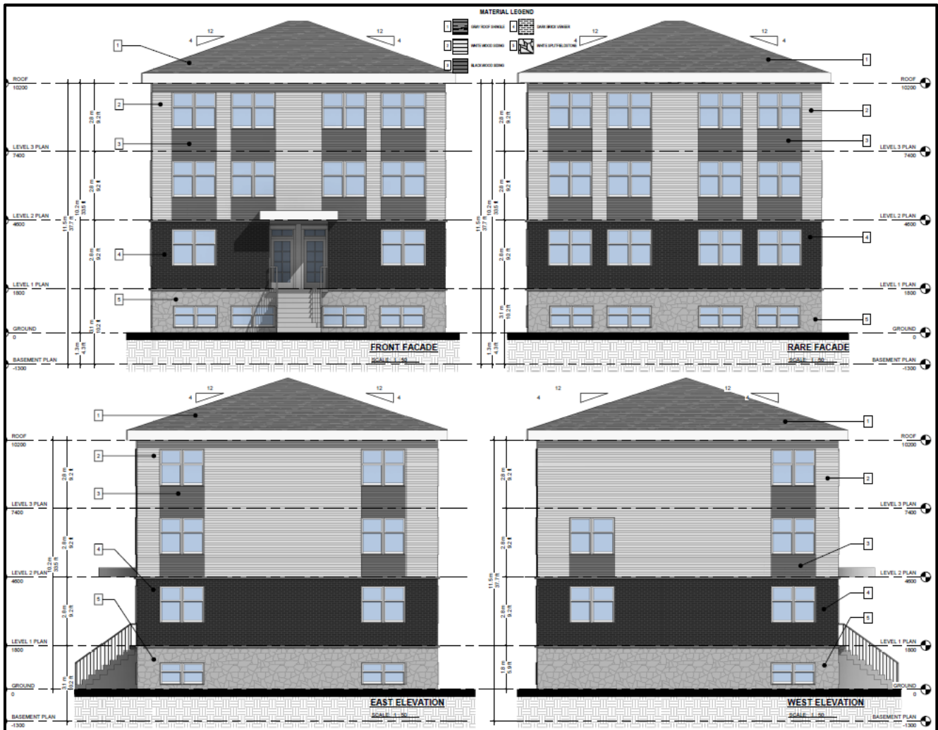
Figure 2. Elevations of Proposed Development.
