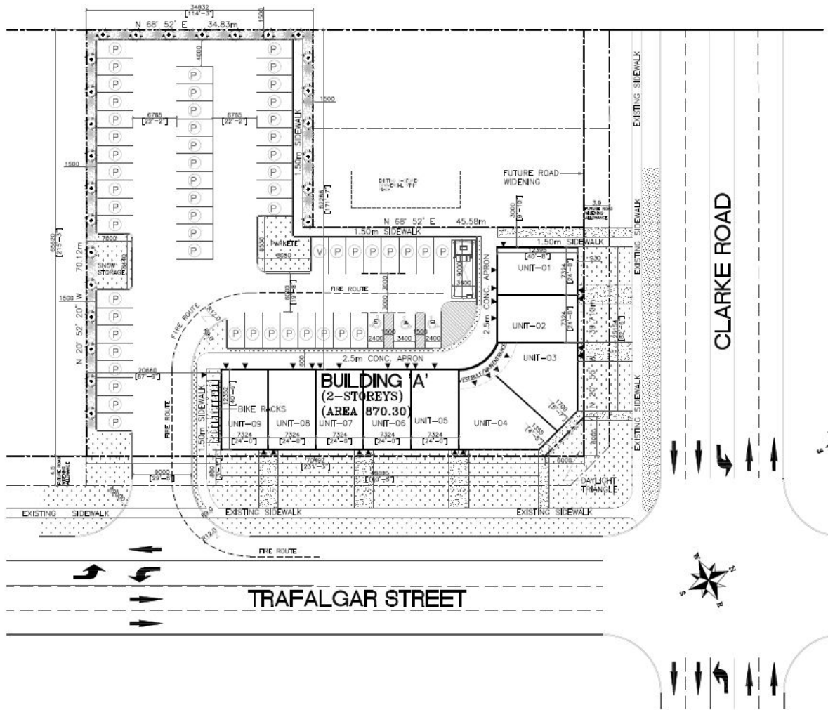
Site Plan
