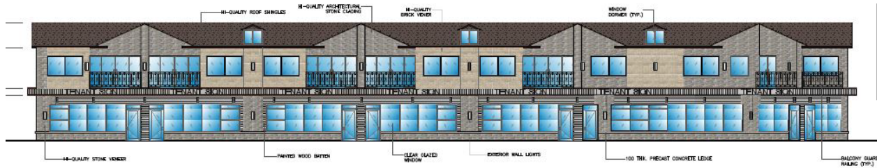
BUILDING FRONTAGE ELEVATION
