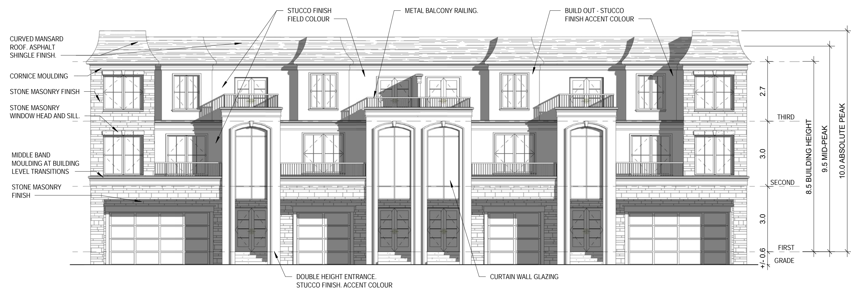
TYPICAL INTERNAL THREE STOREY BLOCK - FRONT ELEVATION
