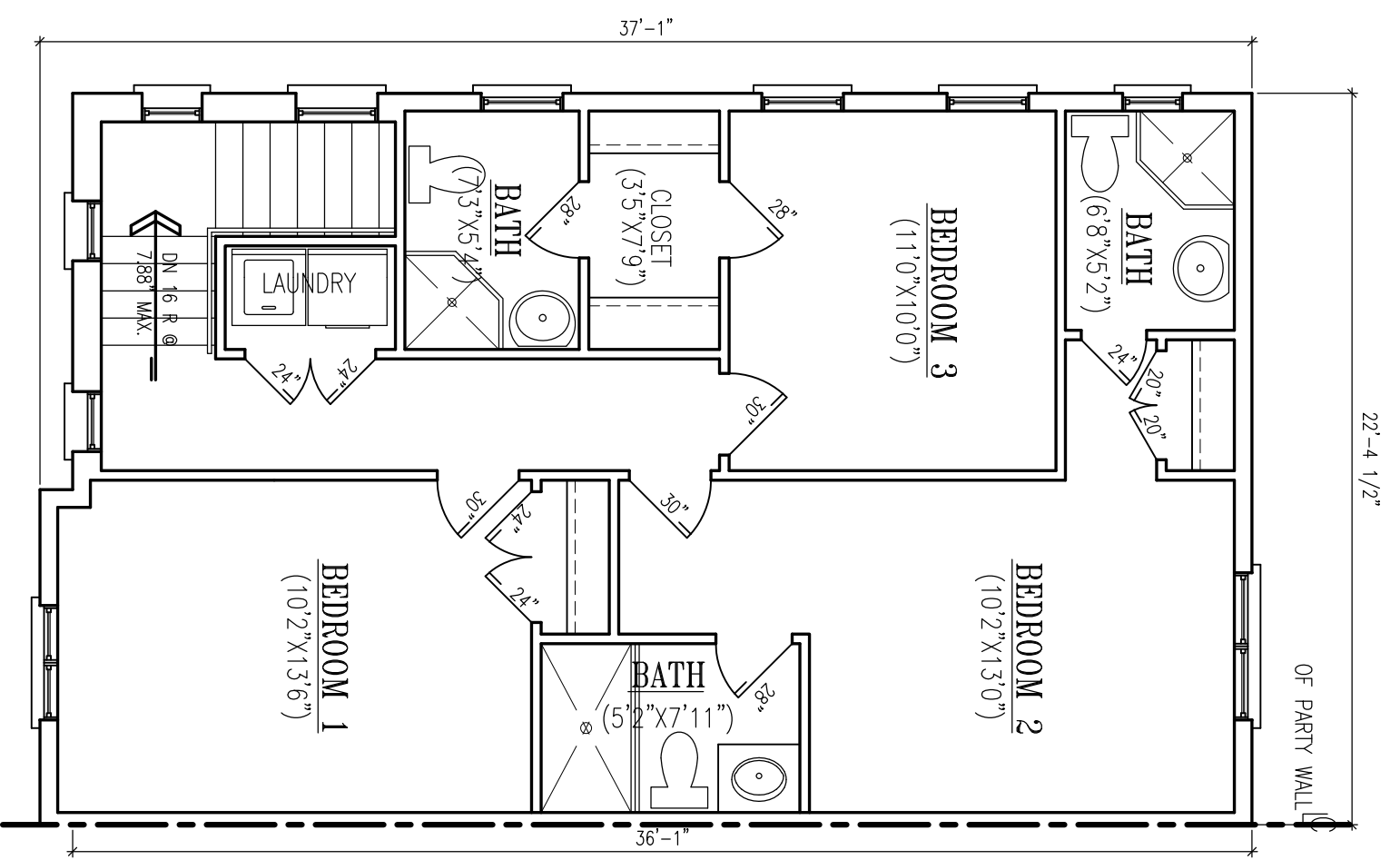
UPPER FLOOR PLAN-CORNER UNIT 818 SQ. FT. 16 WETHERED ST. (APRIL 25/22) 8 UNIT BUILDING
