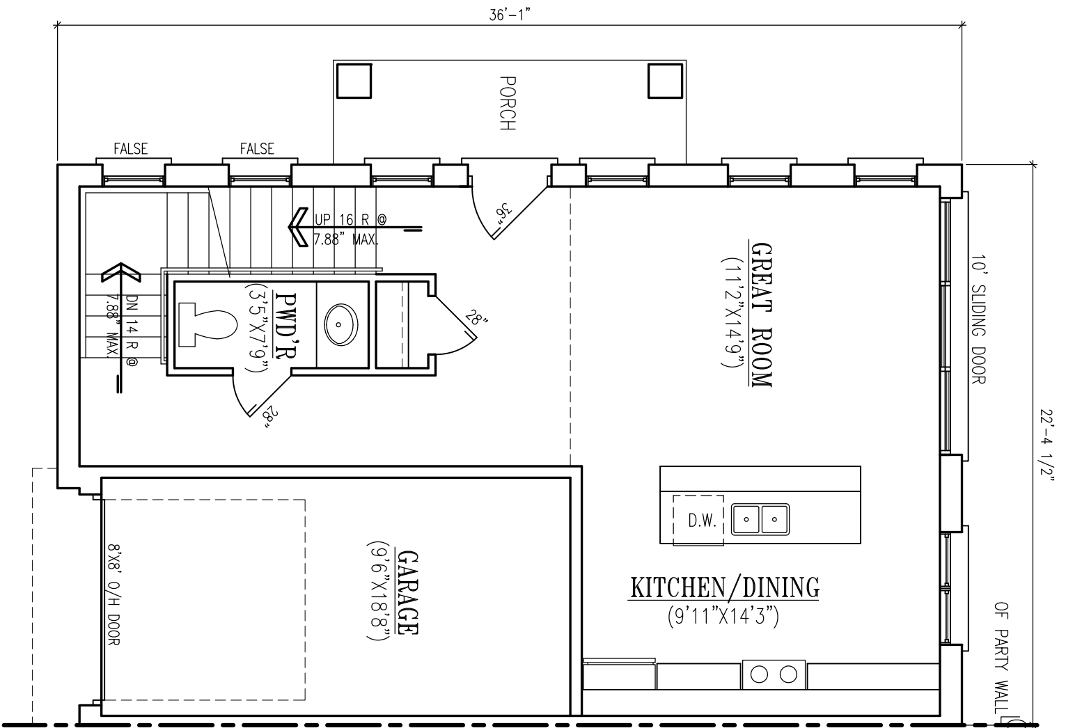
MAIN FLOOR PLAN-CORNER UNIT 605 SQ. FT. (1423 SQ. FT. TOTAL) 16 WETHERED ST. (APRIL 25/22) 8 UNIT BUILDING
